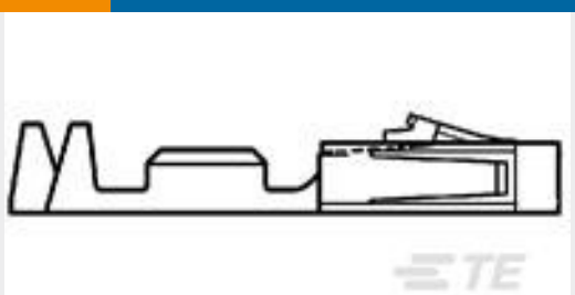
TE 产品编号1-104479-3 SHORT POINT RECP CONT LP
