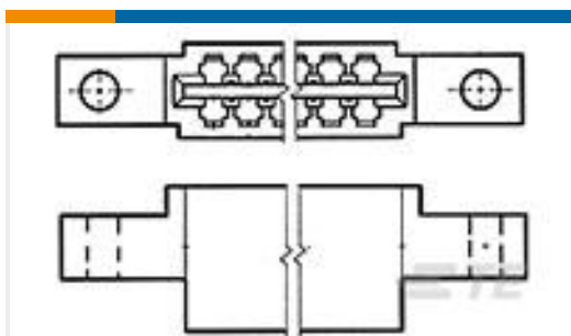
TE 产品编号480110-2 HSG AMP LEAF 15 POS
