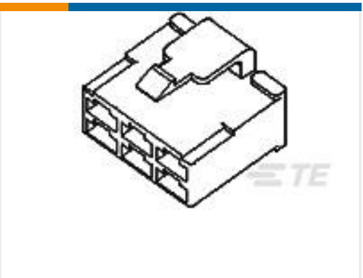
TE 产品编号172134-6 FF 250 PLUG HSG 4P NYLON GRAY
