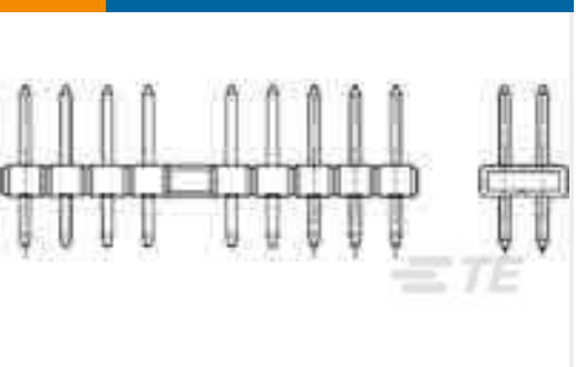
TE 产品编号5176264-9 AMPMODU 2MM V 20P AU:0.2 BLACK LF
