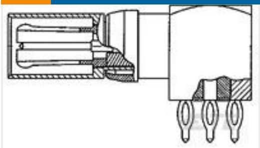
TE 产品编号148386-1 TYPE C,PIN ASSY.RTANG, RF
