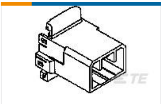
TE 产品编号174931-1 070 MLC W-W CAP HSG 8P NATURAL
