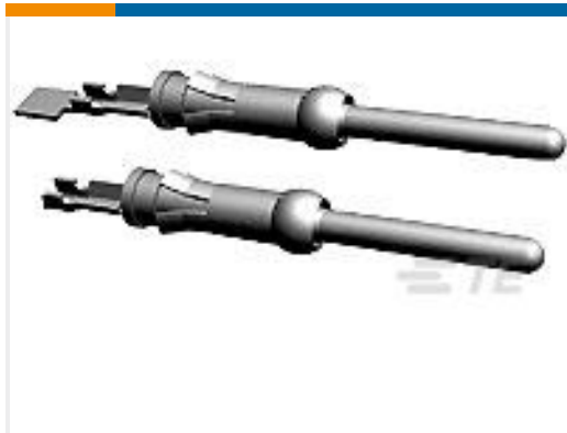
TE 产品编号1-66103-7 III+ PIN,24-20,15AU/FL,SMPACK
