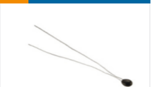
TE 产品编号GA10K4A1D DISCRETE 10K OHMS,+/-1.0C FROM 0C TO 70C
