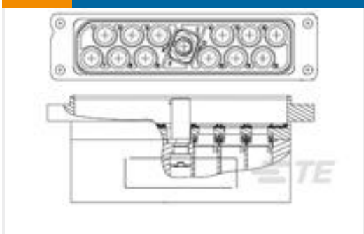
TE 产品编号1604799-7 PANEL MOUNT RECPT,12 POWS,EN PLTD,W/HDWE
