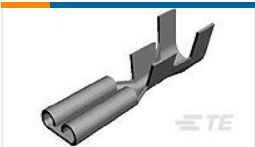
TE 产品编号170203-2 187 FASTON, REC., 24-20 AWG, TPBR
