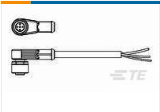
TE 产品编号1-2273012-3 M8 x 1.0 Angled socket Pigtail LED
