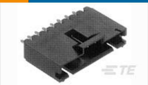
TE 产品编号1375820-8 CST-100 II HOUSING 8 POS
