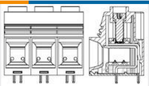
TE 产品编号1986242-5 Power Connector, 15.0mm, Green, 5 posn
