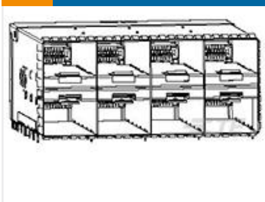
TE 产品编号1-2180324-9 zSFP+ STACKED 2X4 RECEPTACLE ASSEMBLY
