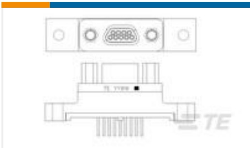
TE 产品编号1532266-2 M83513/22-A01CP = MCKS-C2-P-9PST1
