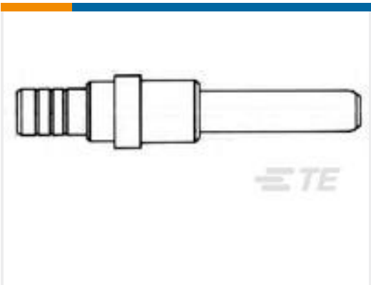
TE 产品编号1738025-1 Pin Contact,Size 15
