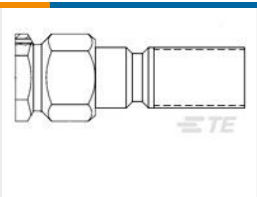
TE 产品编号1051817-1 SMA CABLE PLUG 2031 8162 92
