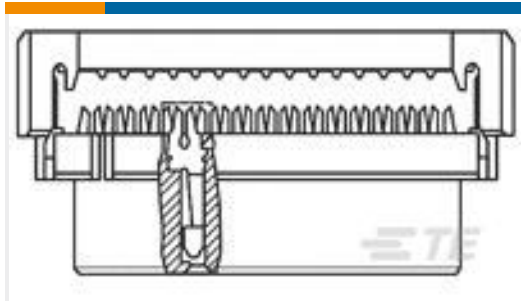
TE 产品编号1-111626-9 20, 2MM, 30 DP, LEAD FREE
