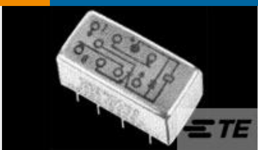
TE 产品编号3-1617073-8 3SBC2096A2 = M39016/37-026P
