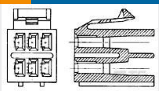
TE 产品编号103366-2 06 MODI CRMP S-I HSG DR .156CL
