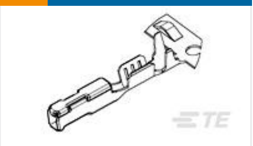
TE 产品编号1456968-1 CONTACT,FEMALE, 0.64, 20 TO 22 AWG, AG
