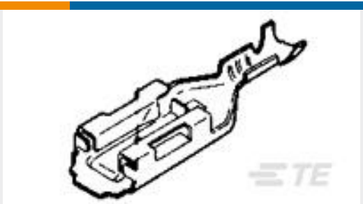
TE 产品编号170452-1 PL 250 AM REC 22-20 AWG 0.406 X 21 BR
