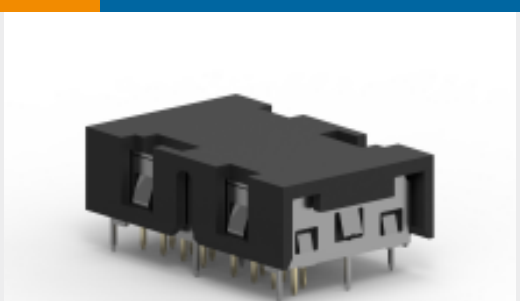
TE 产品编号1-2208264-3 POF,FO PIGTAIL,MOST,FOT UNIT, ASSY
