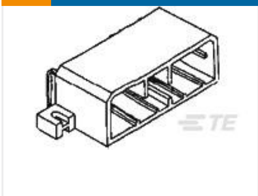
TE 产品编号1747997-1 CAP HOUSING ASSY 14POS 1.8 SERIES MLC I/
