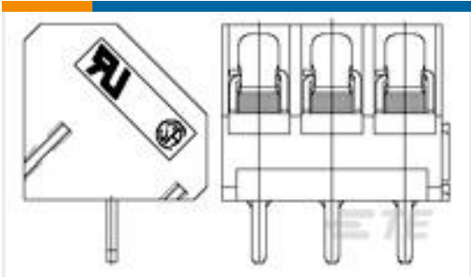
TE 产品编号1776252-2 45 degree wire inlet, 5.0mm, H
