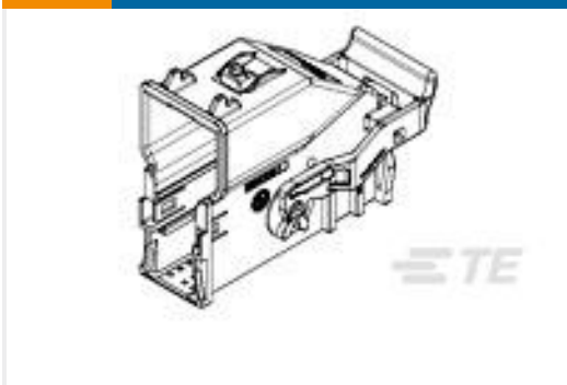
TE 产品编号1-1924337-3 Shield Assy, 54 POSN, 0.64mm, 20 DEG BLK
