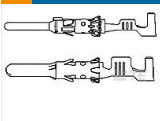
TE 产品编号1703013-4 DIA 1.5MM CONTACT PIN,ASSY
