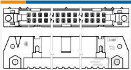
TE 产品编号102142-7 UNV AMP-LATCH HDR HSG 60P W /MTG EARS
