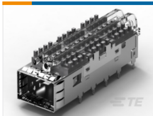
TE 产品编号2-2170705-4 CAGE ASSY, QSFP28 1X1, SPRING, HS, LP
