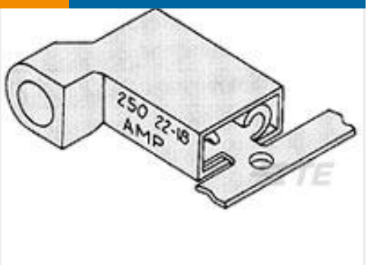
TE 产品编号3-520338-2 ULTRA-FAST 187 ASY REC 16-14 AWG TPBR
