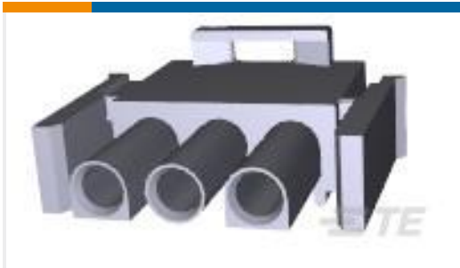
TE 产品编号1-480700-0 03P UMN2 PLUG HSG NATL
