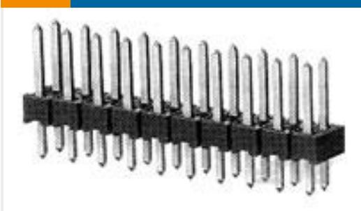
TE 产品编号8-146252-2 64 MODII HDR DRST B/A .100 LF
