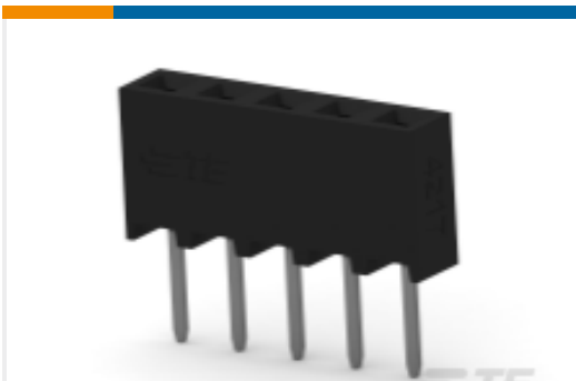
TE 产品编号2314878-5 5P,2MM,B-B,REC,SRVT,2.7,0.76AU,TB
