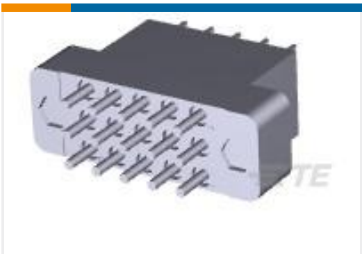
TE 产品编号205628-3 AUTOWIRE KIT, 15 POS, 25 X 25
