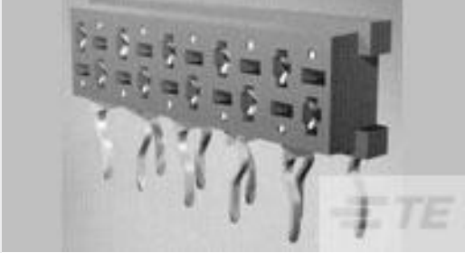
TE 产品编号1-100400-6 MICRO-MATCH FSID NP
