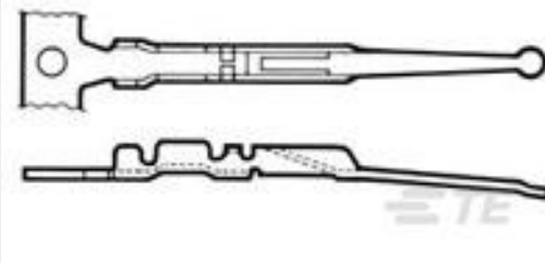
TE 产品编号66750-2 CONT,CR,ACTIVE FOR 22 AWG WIRE
