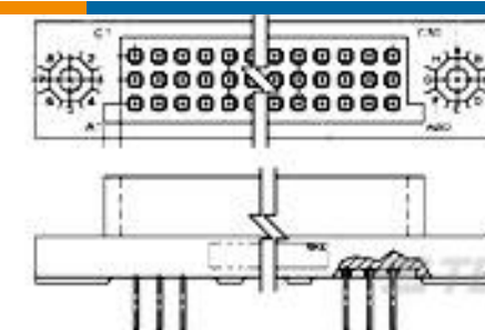
TE 产品编号446853-5 3ROW BOX REC 165P 100CLSEALED
