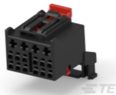
TE 产品编号1-2295393-1 PLUG ASSY, 16WAY, HYBRID, UNSEALED, A
