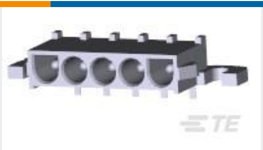
TE 产品编号1-350945-0 05P UMNL HDR ASSY R/A 94VO
