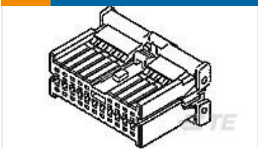
TE 产品编号1123371-1 040-3 MLC PLUG HSG ASSY 16P
