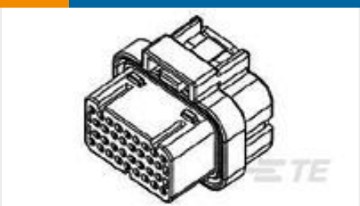
TE 产品编号3-1437290-8 26POS,SUPERSEAL,REC HSG ASSY, SLD,COD 2
