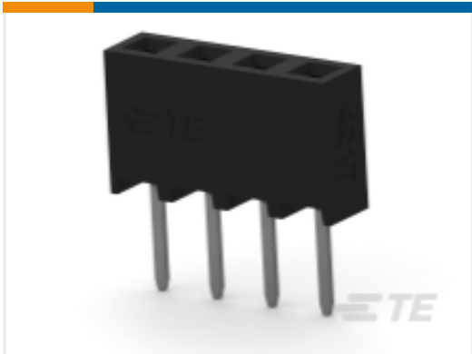
TE 产品编号2314878-4 4P,2MM,B-B,REC,SRVT,2.7,0.76AU,TB
