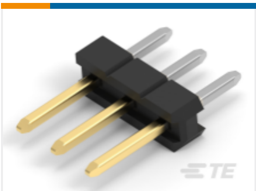
TE 产品编号2355182-4 4P,2MM,BRK HDR,SRVT,2.8,0.76AU,TB
