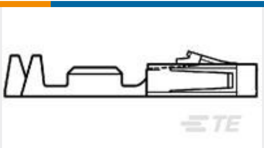
TE 产品编号104479-3 SHORT POINT CONT 15 DPLX STMPD
