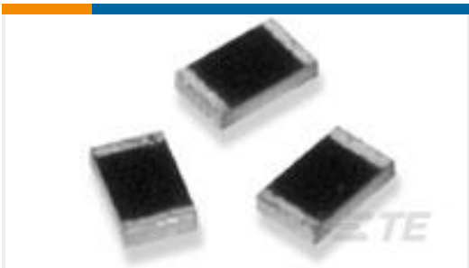
TE 产品编号1625868-6 RP 2A 0.25W 200R 0.1% 25PPM 1K RL
