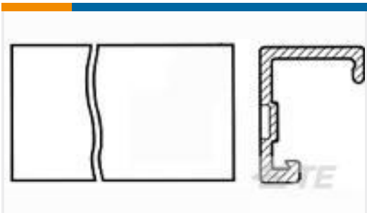
TE 产品编号1-640551-8 18P MTA156 COVER
