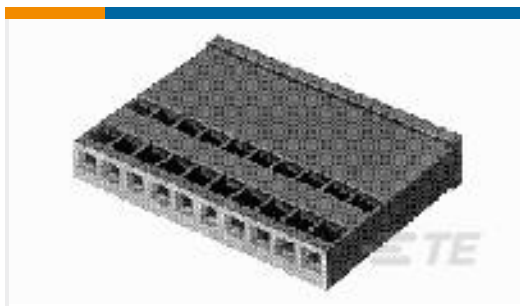
TE 产品编号 2-87175-2 10 LOCKING CLIP HSG SR .100CL
