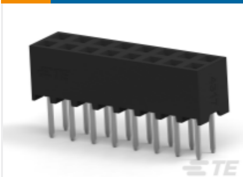
TE 产品编号1-2314824-6 16P,2MM,B-B,REC,DRVT,2.7,0.1AU,TB, W/CAP
