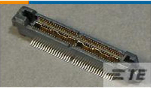
TE 产品编号 767116-2 MICT,260PLG,076,ASY,.025,AUPLT
