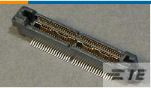
TE 产品编号 767111-9 MICT,PLG,076,ASY,.025 TAPE CAP
