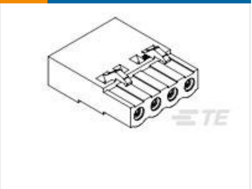
TE 产品编号1986160-5 Crimp Style housing, 5.08, Green, 5 posn
