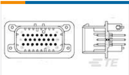
TE 产品编号1-776228-2 HEADER ASSY, 23 POS VERTICAL
