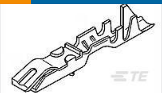
TE 产品编号5-87165-2 LOCKING CLIP ASSY .025 SQ LP
